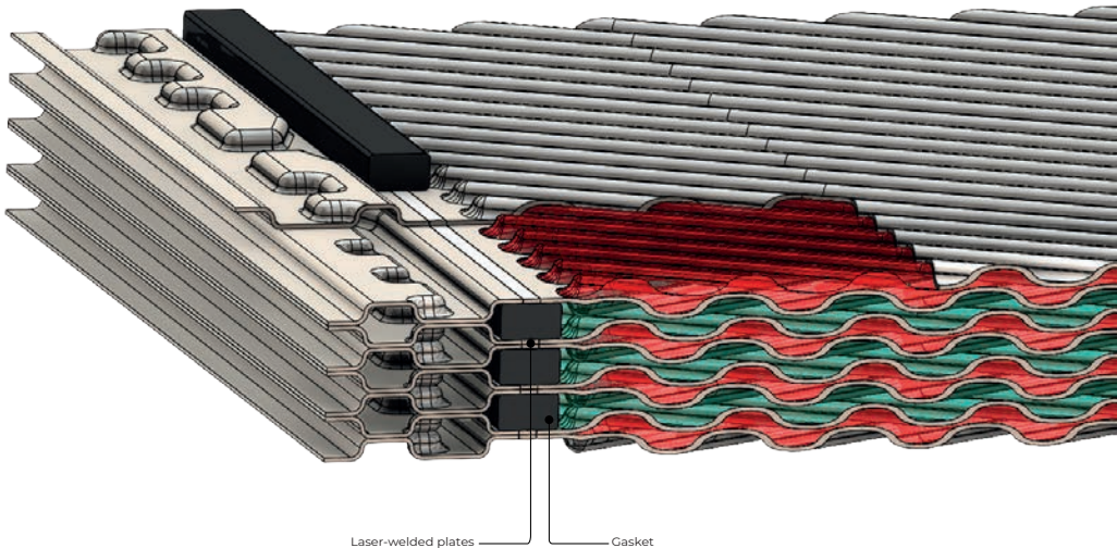
Laser-welded plates
